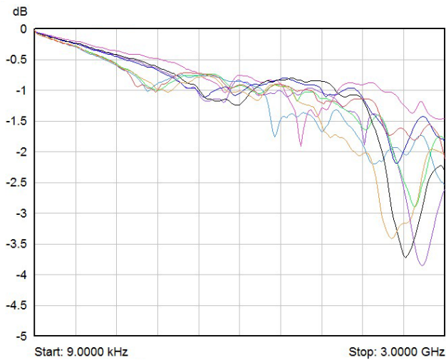
40-710-514 (50 \Omega SMB) typical insertion loss plots for all NO and NC inputs.
