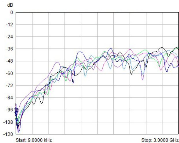
40-710-514 (50 \Omega SMB) typical crosstalk plots between neighbouring channels.
