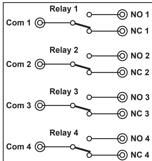
Switching Diagram for 40-710, 4 x SPDT RF Relays
