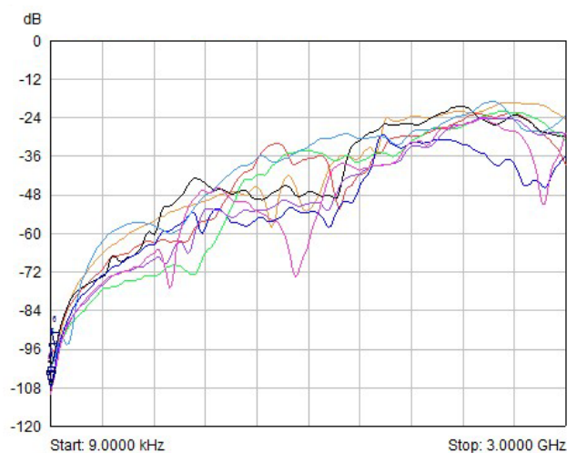
40-710-514 (50 \Omega SMB) typical isolation plots for all NO and NC inputs.
