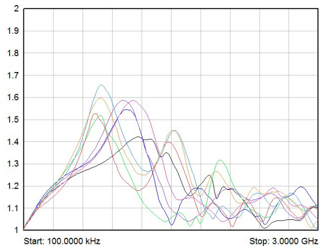
40-710-514 (50 \Omega SMB) typical VSWR plots for all NO and NC inputs.
